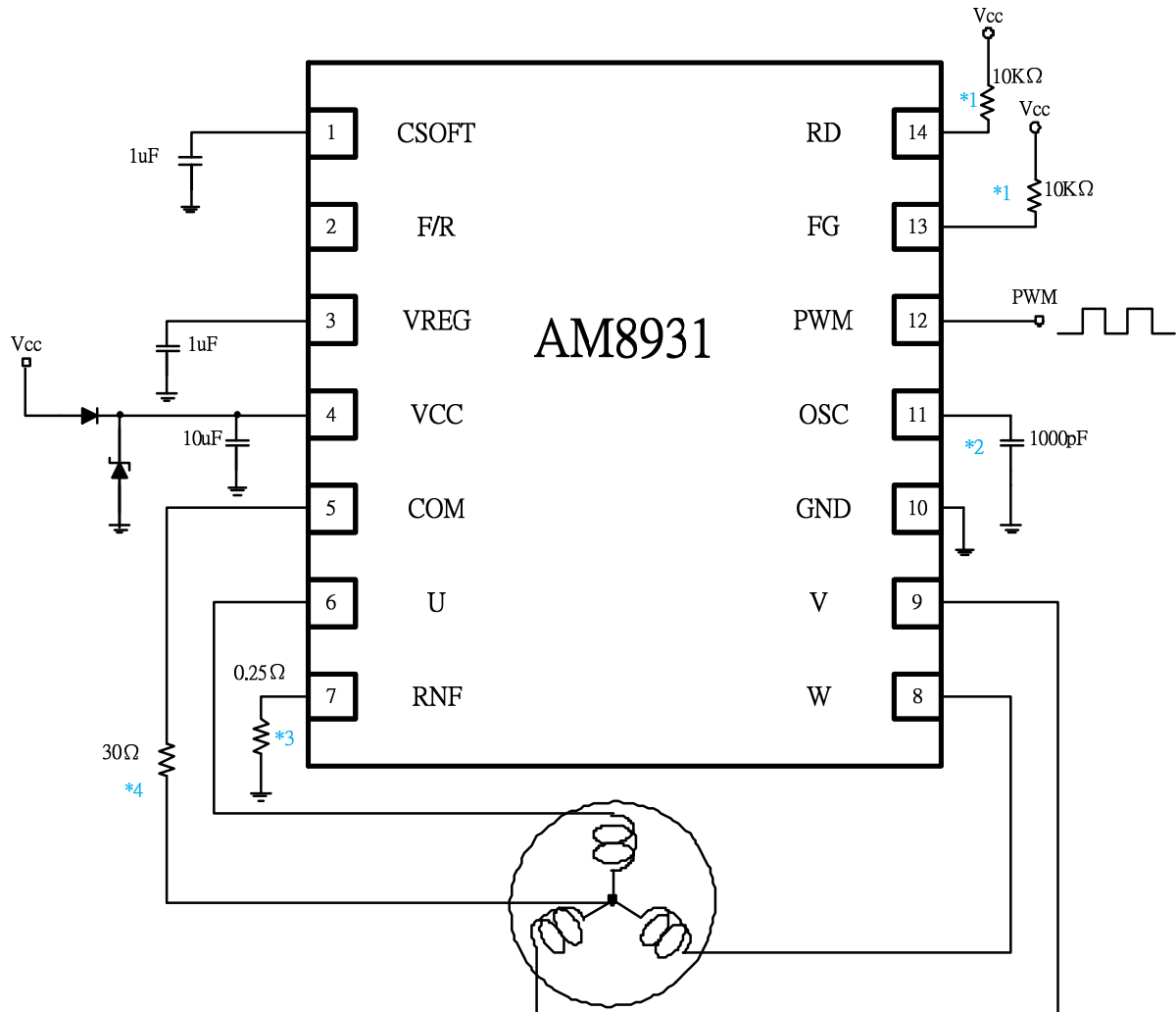
Fig.2 Application circuit
