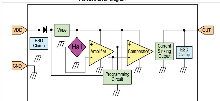
Function Block Diagram
