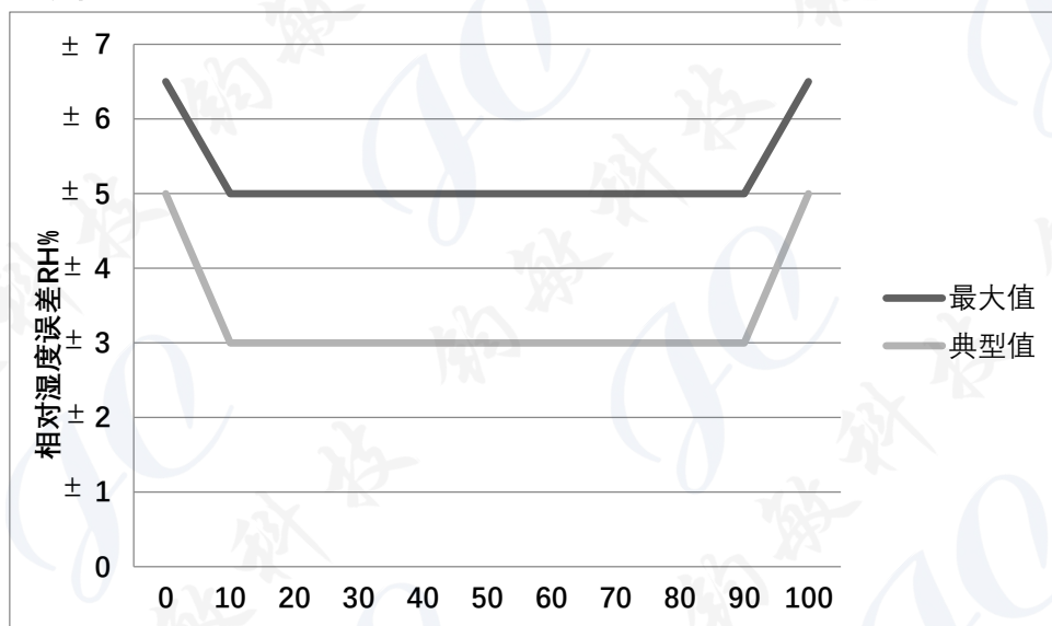
图 3 Tolerance of RH at 25°C for GXTH30
