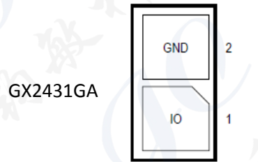
SFN (3.5mm x 6.5mm x 0.75mm)
