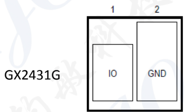
SFN (6mm x 6mm x 0.9mm)
