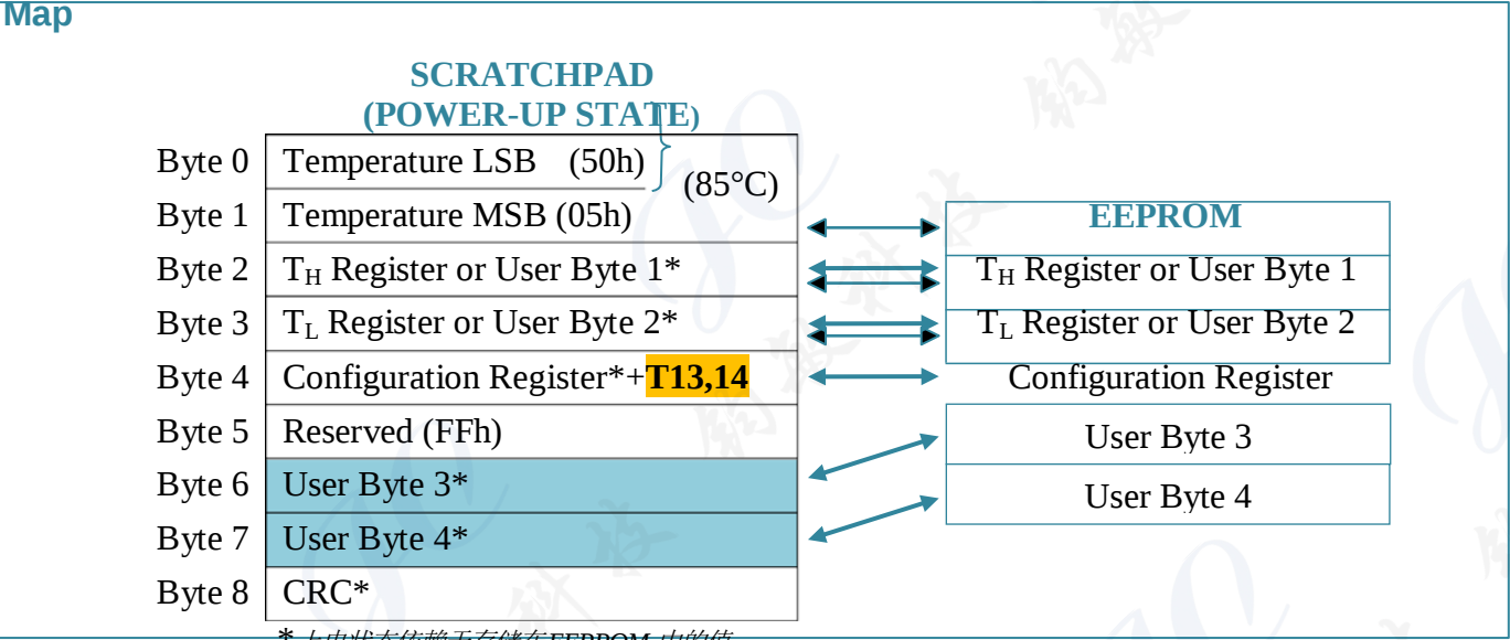
Figure 7. GX20MH01 Memory Map
