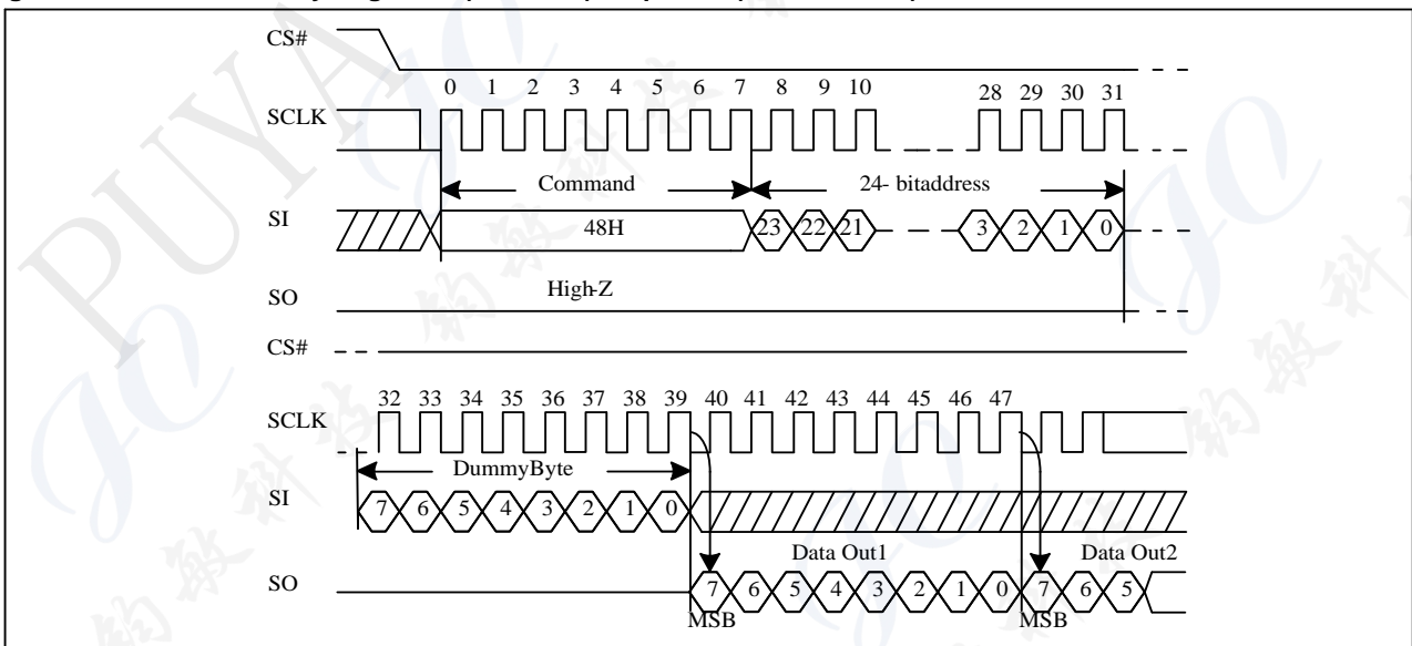
Figure 10-27 Read Security Registers (RDSCUR) Sequence (Command 48)
